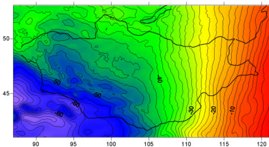
Figure 14 - Computed gravimetric quasigeoid of Mongolia.
