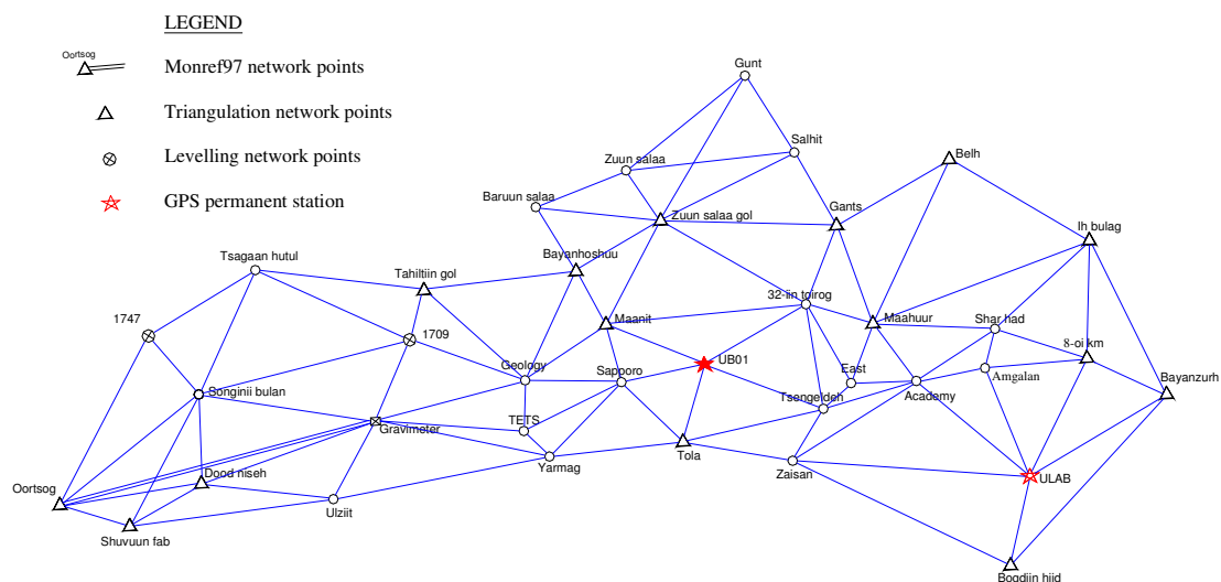
Figure 7 - GPS network of Ulaanbaatar city
