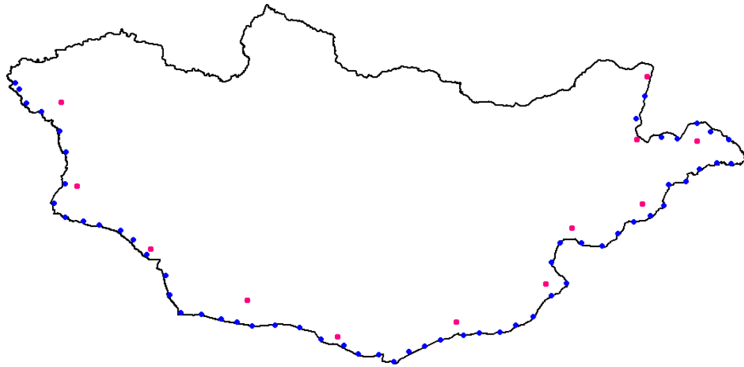
Figure 8 - GPS network established along Mongolian-China border line
