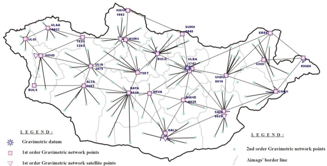
Figure 2 - Gravity network of Mongolia
