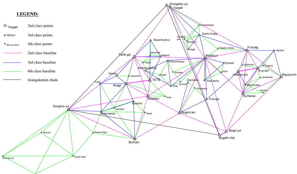
Figure 4 – Ulaanbaatar city's triangulation network
