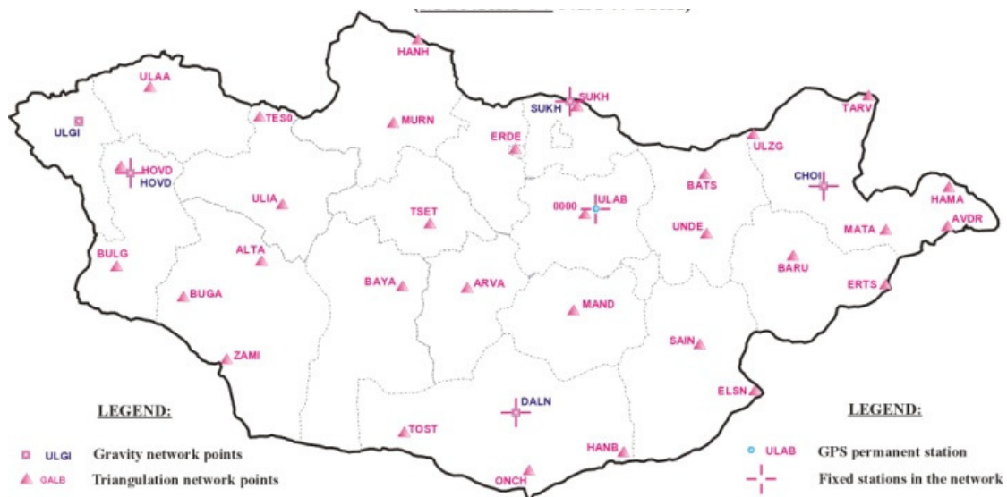
Figure 5 - GPS network of Mongolia /Monref97/
