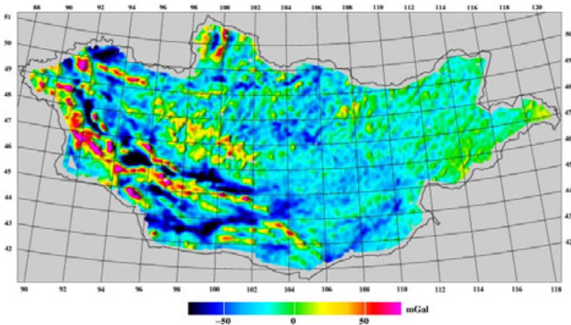
Figure 13 - Airborne free-air anomalies at altitude from airborne gravity survey. Colour scale is from -75 to 75 mGal.
