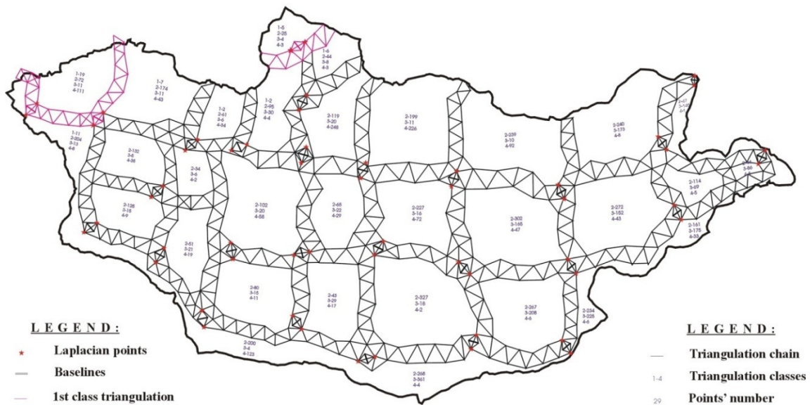
Figure 1 - Triangulation network of Mongolia
