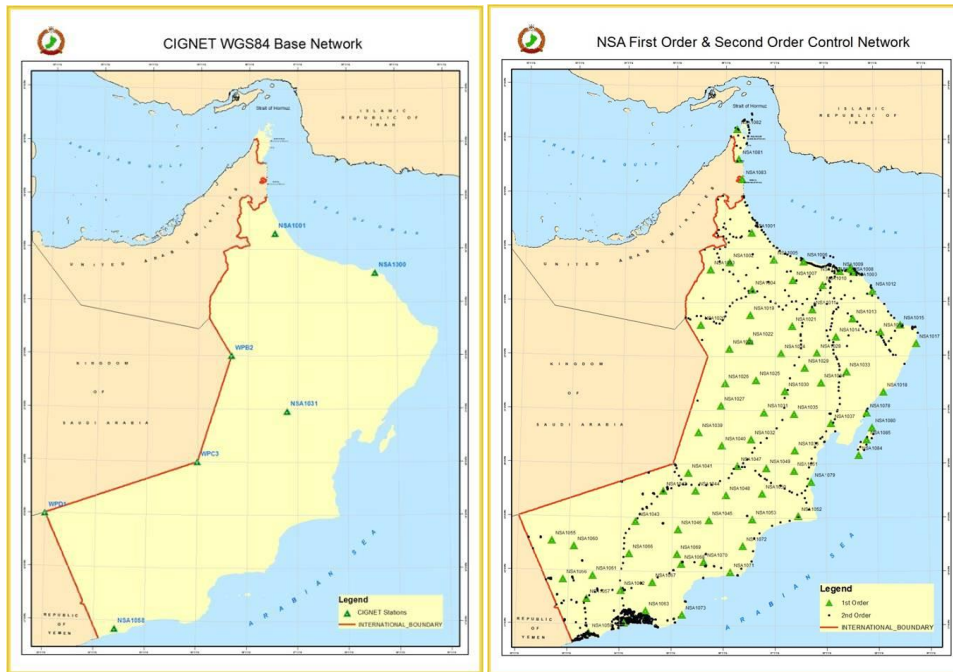
Figure 1: CIGNET WGS84 Base Network and the First and second order GPS station in Oman (NSA, 2014)
