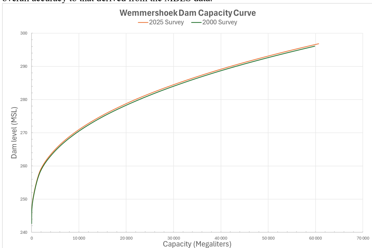
Figure 12. Capacity curves.
