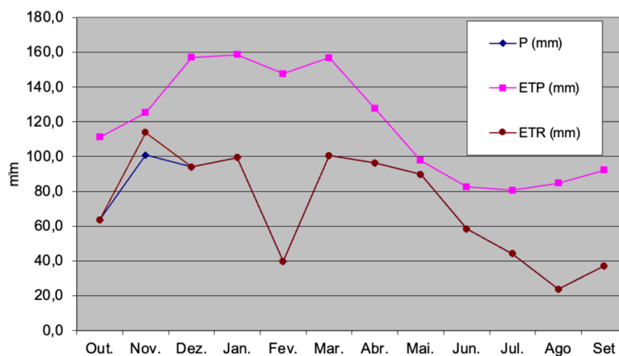
Figure 3 - Hydrometeorological Water Balance of the Municipality of Armação dos Búzios - RJ
