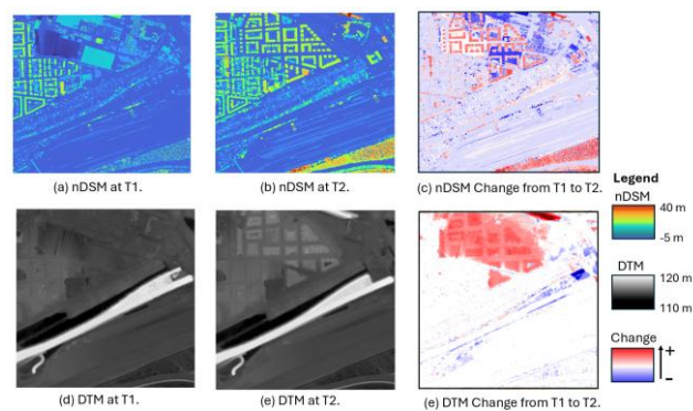
Figure 5 – nDSM change and DTM change between the timestamps T1 (2001) and T2 (2016) for a spatially selected part of Karlsruhe.
