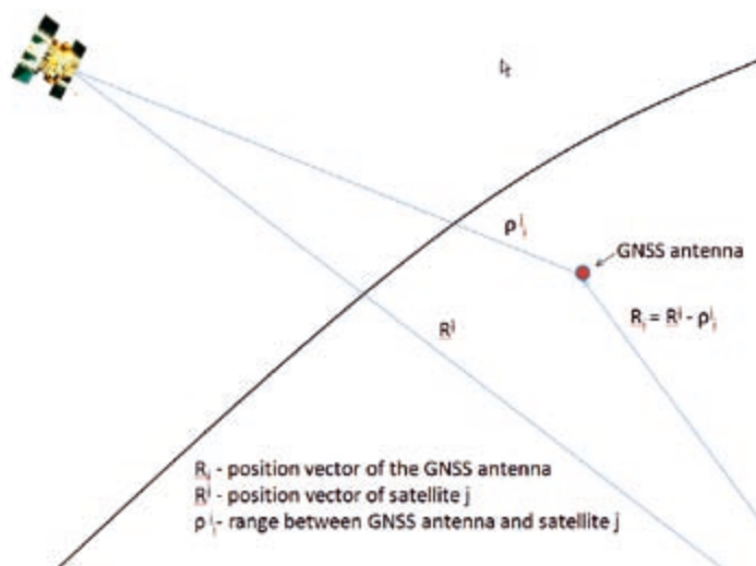
Fig. 1: Satellite positioning using an ECEF reference frame.
