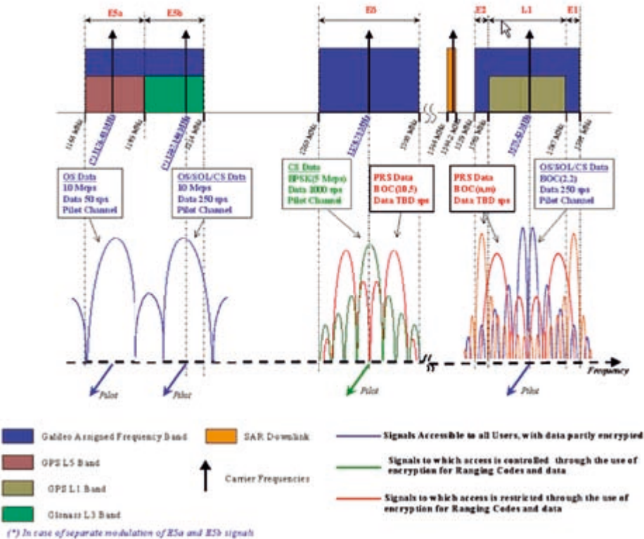
Fig. 2: Galileo Signal Structure. (Courtesy Institute of Geodesy and Navigation, University FAF Munich)
