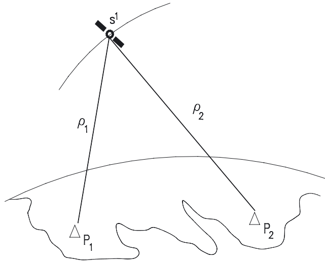
Fig. 4: Single-difference.
