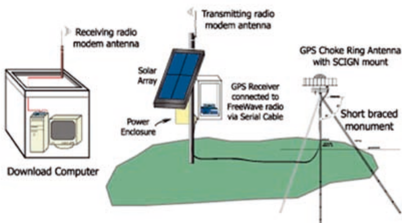
Fig 14: Typical CORS station configuration for the Plate Boundary Observatory (PBO) network. Courtesy UNAVCO, CO.
