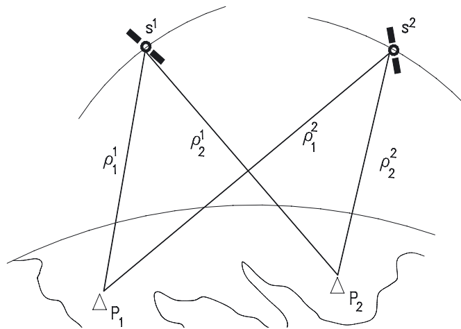
Fig. 5: Double-difference.
