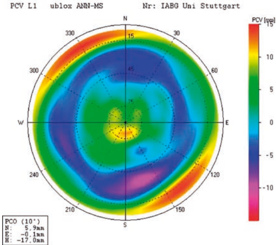
Fig. 11: Antenna pattern for u-blox ANN-MS antenna.
